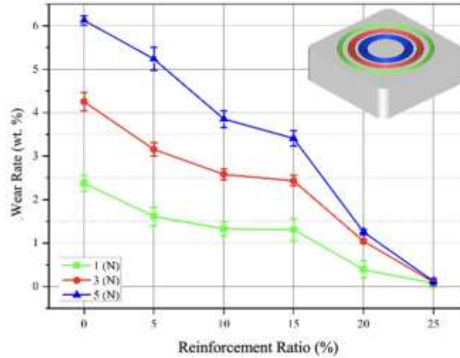
Figure 2. Effect of PPA content on wear loss (%) under normal loads of 1, 3, and 5 N.
