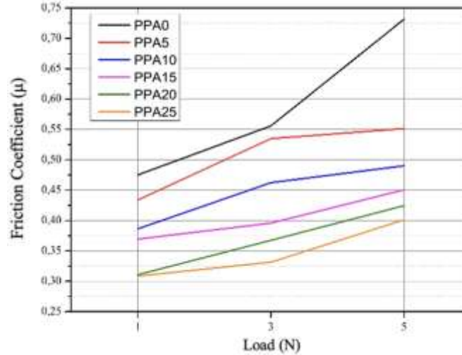
Figure 5. Effect of PPA content on the coefficient of friction of the developed brake pad composites under normal loads of 1, 3, and 5 N.
