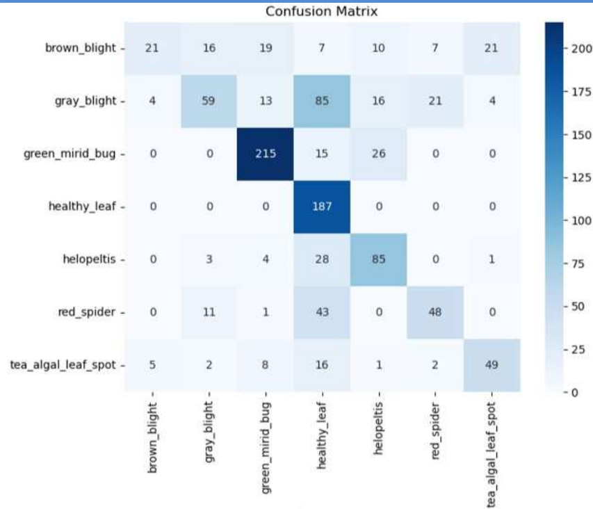
Figure 6. Confusion matrix of proposed model.
