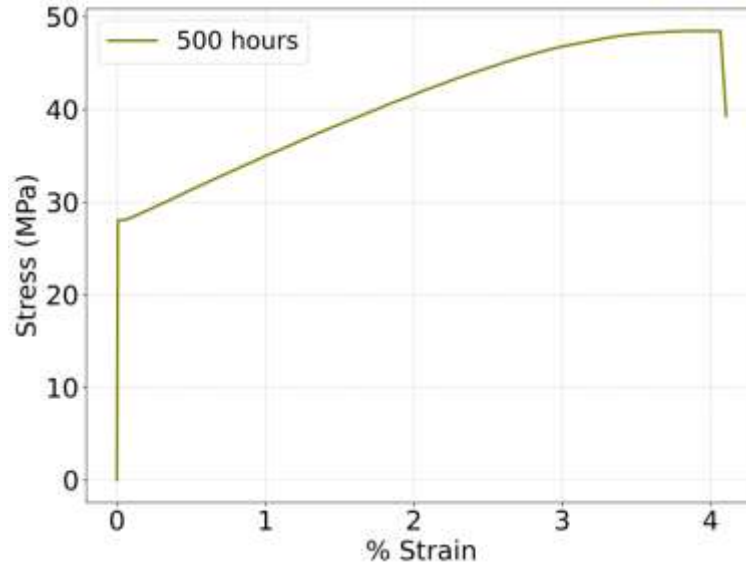
Figure 3 Stress-strain curve of a sample subjected to 500 hours of artificial aging treatment.
