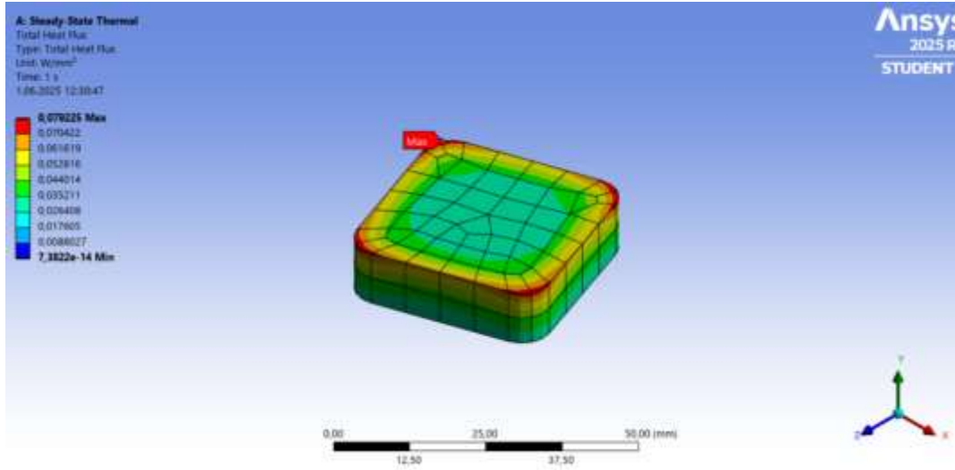
Figure 7. Total heat-flux distribution of the PPA25 brake pad composite obtained from ANSYS Steady-State thermal analysis.
