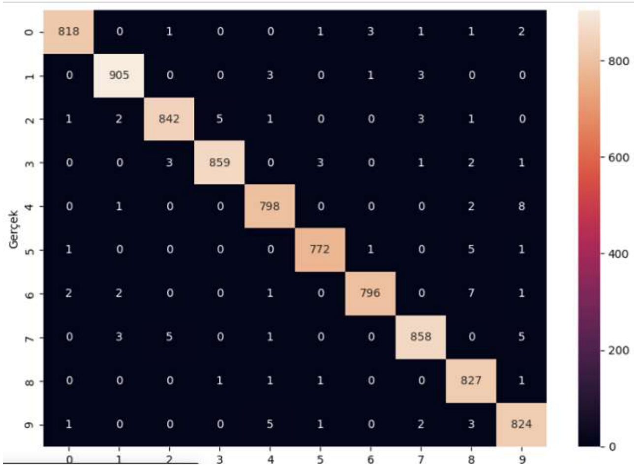
Figure 2: Confusion Matrix of the Model on the Validation Dataset.
