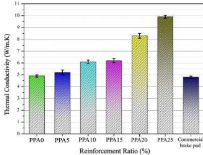
Figure 4. Effect of PPA content on the thermal conductivity of the developed brake pad composites
