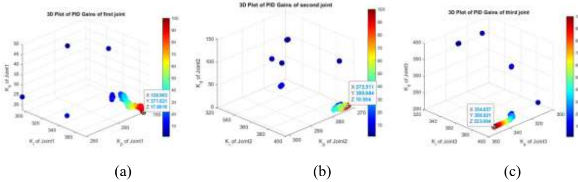
Fig. 8 – 3D Distribution of PID Controller Gains
