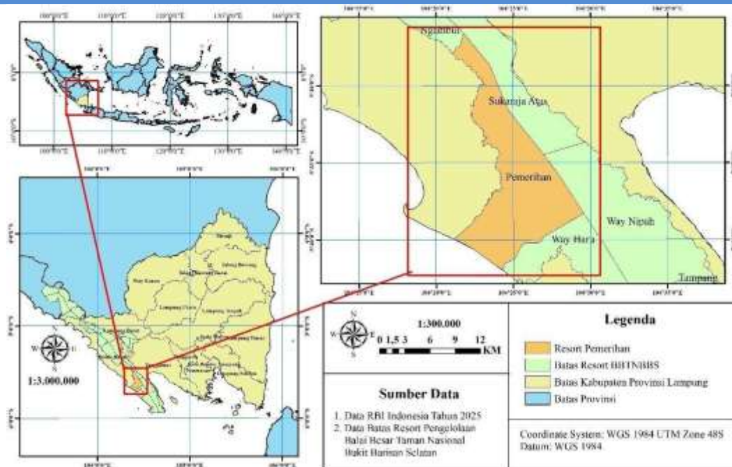
Figure 1. Map of the research area of the Resort of Pemerihan
