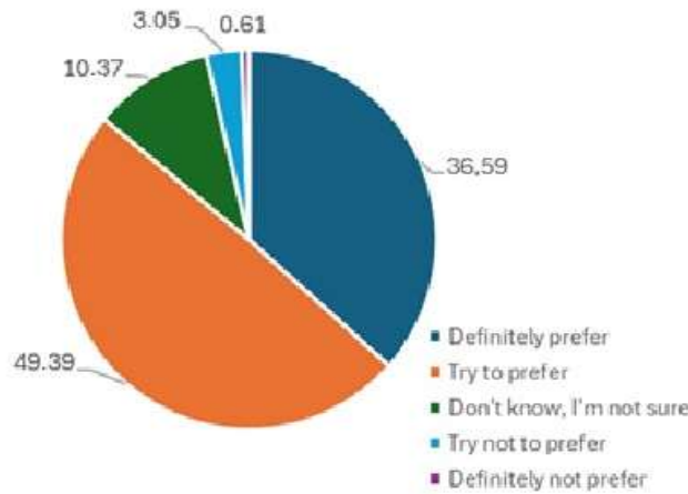
Graph 4: Willingness to pay an entrance fee for national parks.
