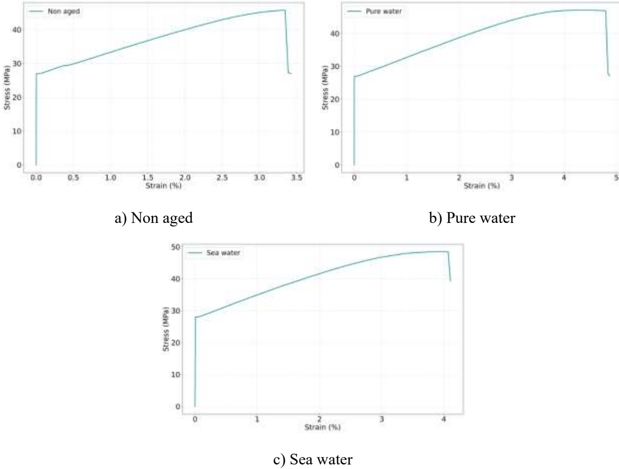
Figure 3 Stress-strain curves obtained from tensile tests of a) non aged, b) pure water, c) sea water condition.
