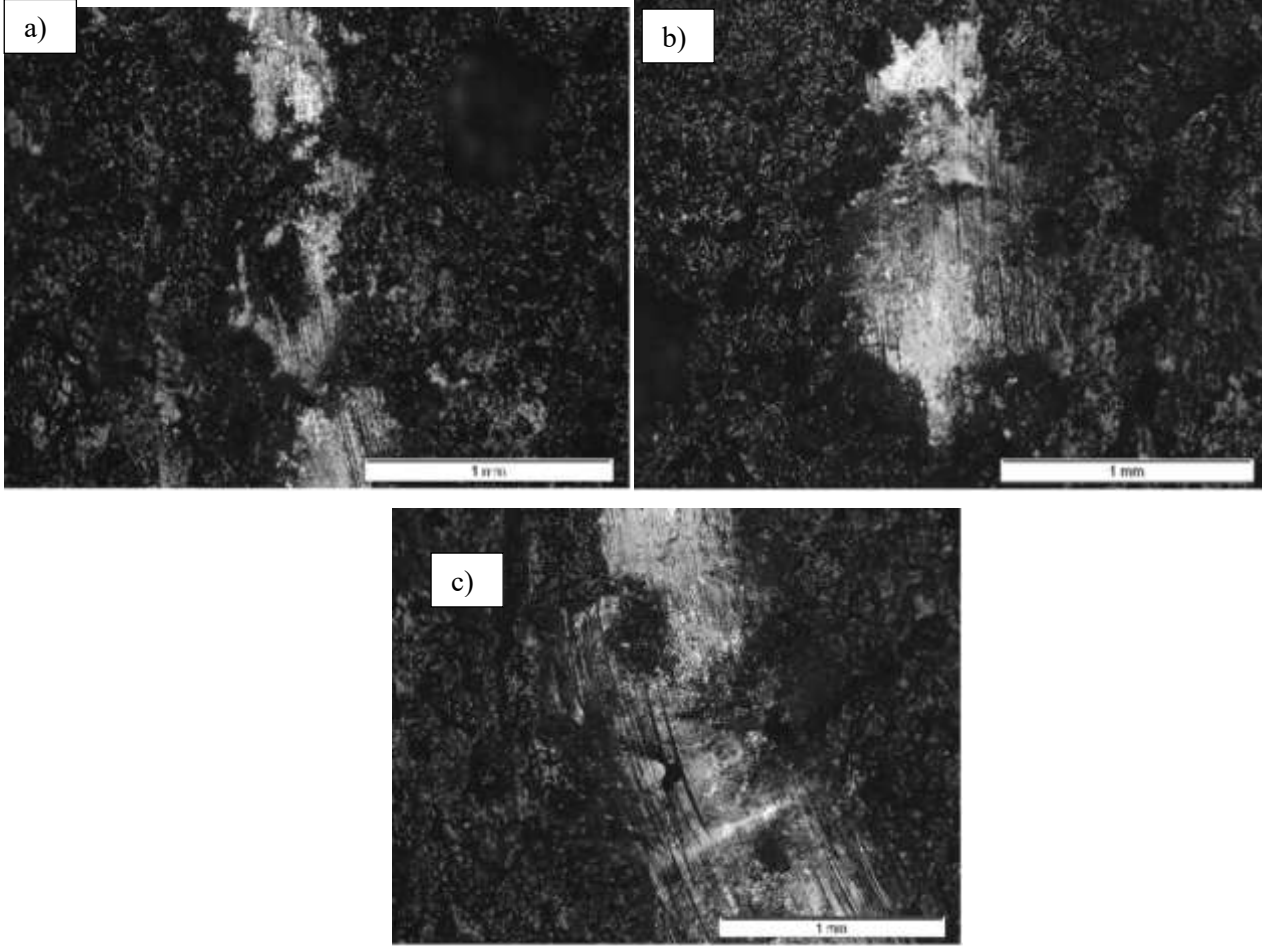
Figure 6. Optical micrographs of the worn surface of the PPA-reinforced composite after wear testing under (a) 1 N, (b) 3 N, and (c) 5 N normal loads
