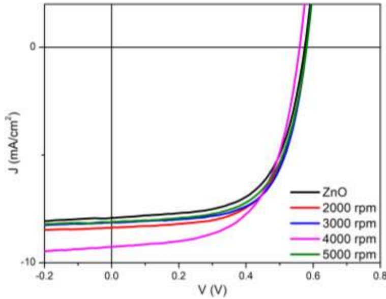
Figure 3. J-V graphs of best devices
