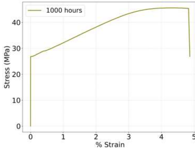
Figure 4 Stress-strain curve of a sample subjected to 1000 hours of artificial aging treatment.
