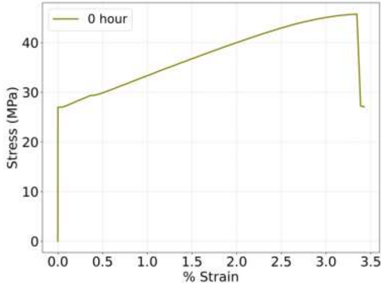
Figure 2 Stress strain curve of a sample not subjected to artificial aging treatment.
