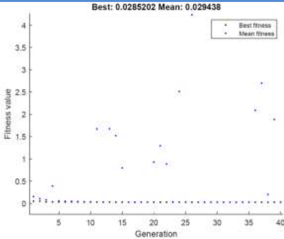
Fig. 7 – Convergence of the Genetic Algorithm/ ITEA technique for PID Position Optimization
