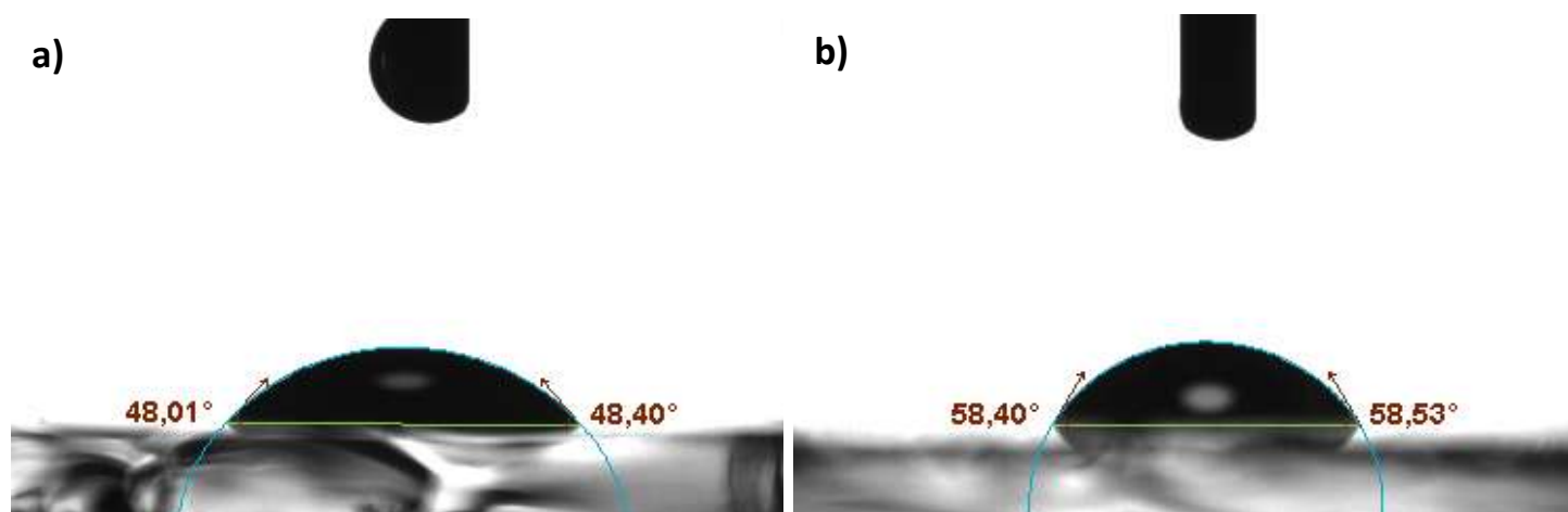
Figure 2. Contac angle measurements of a) ZnO b) ZnO/MBA
