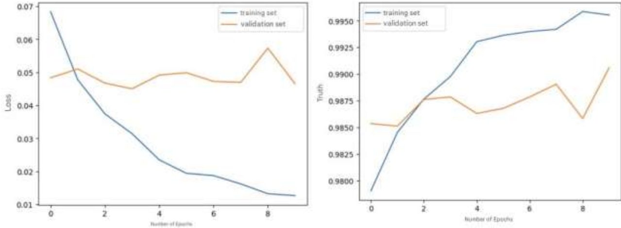
Figure 3: Training and Validation Loss (left) and Accuracy (right) Curves During the Training Process.
