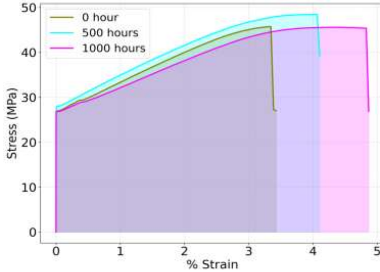
Figure 5 A combined presentation of the stress-strain curves for all samples.
