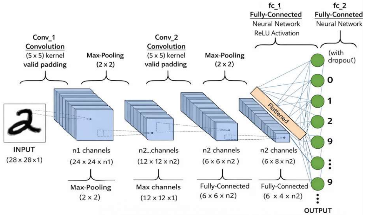
Figure 3. A general CNN architecture used in image processing
