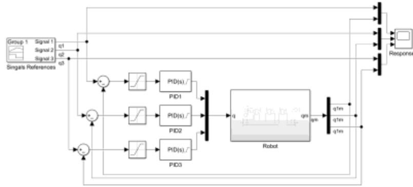
Fig. 4 – PID controller with singles references.
