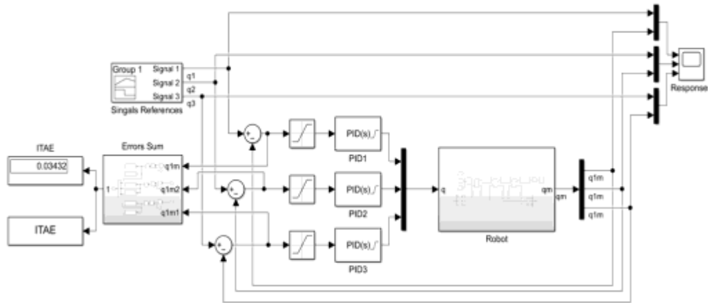
Fig. 5 – Errors sum of ITEA
