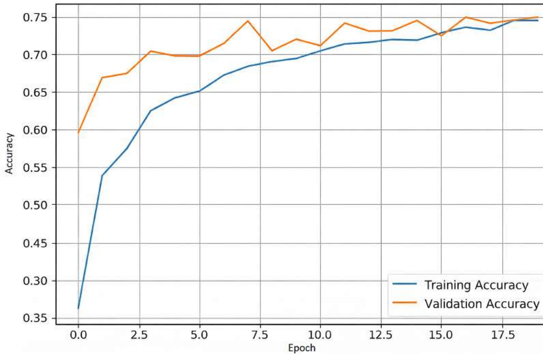
Figure 5. Training and Validation Accuracy over Epochs.
