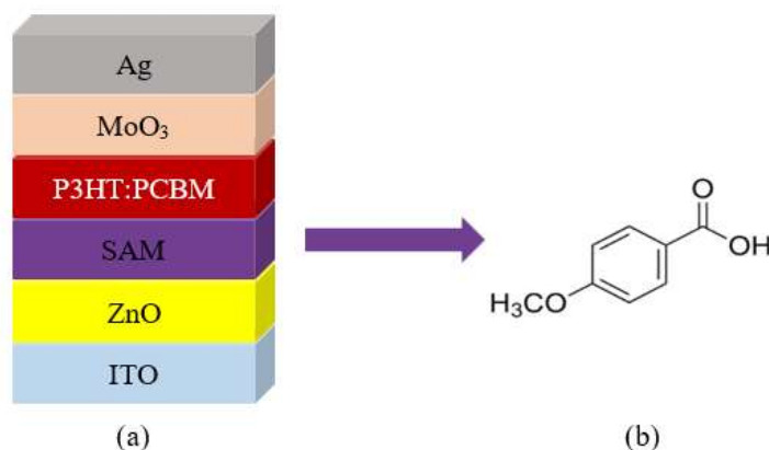
Figure 1. a) Schematic representation of the produced device b) Molecule structure of MBA
