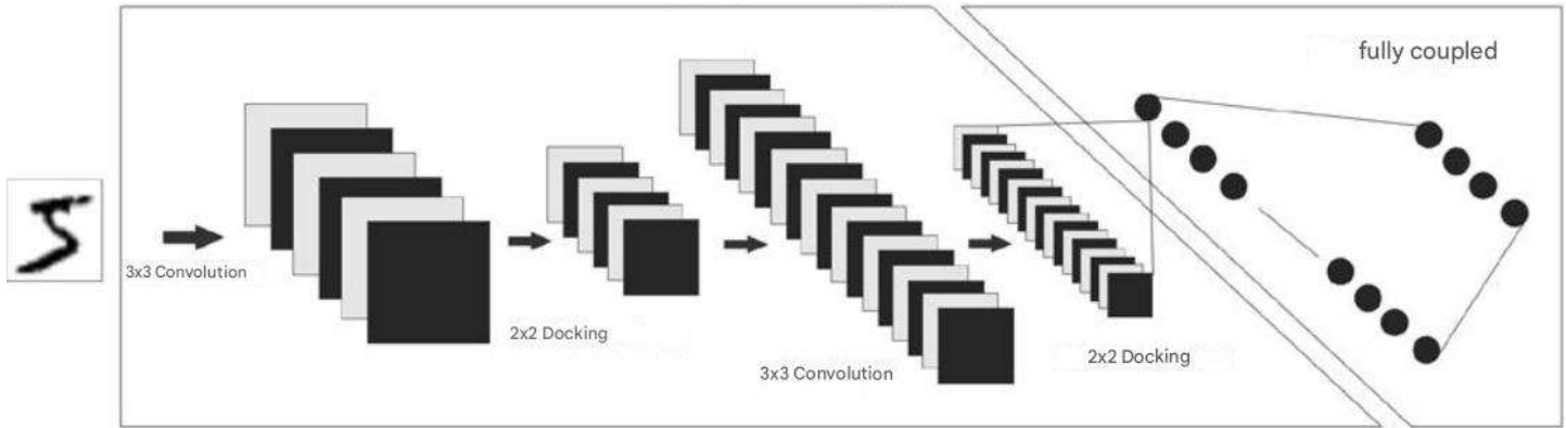
Figure 1: Typical CNN Architecture Showing Convolution, Pooling, and Fully Connected Layers.
