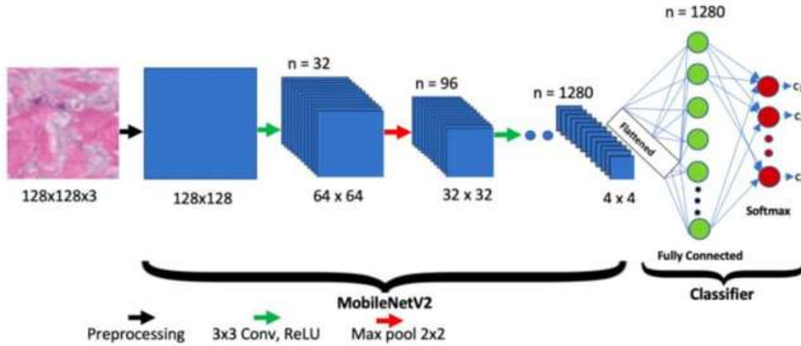
Figure 4. Proposed MobileNetV2 architecture.
