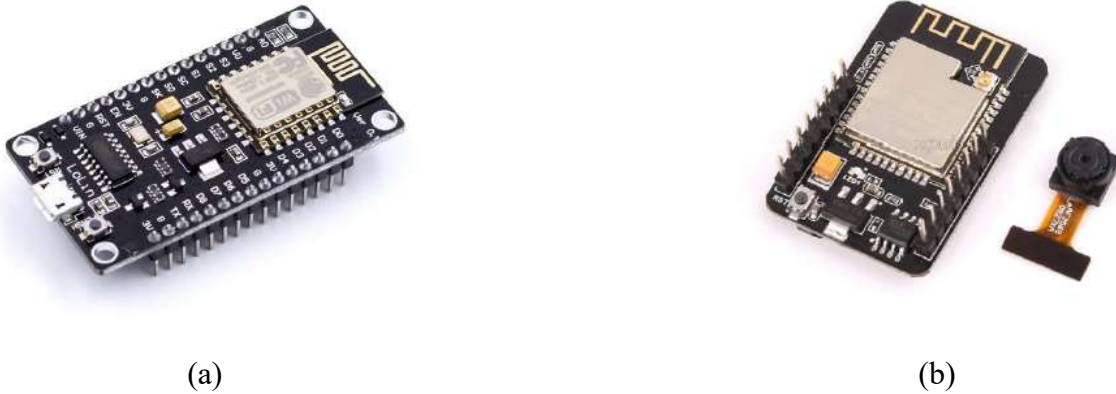
Figure 4. Hardware components used in the proposed system: (a) ESP8266 module and (b) ESP32-CAM module.
