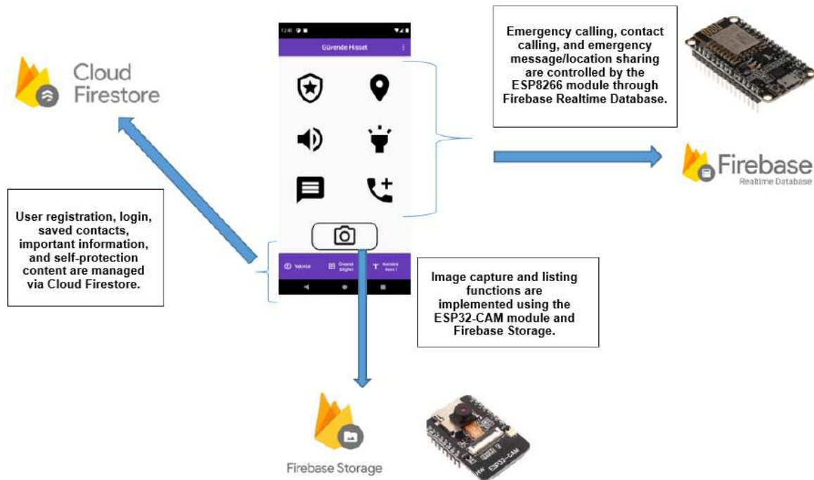
Figure 5. Overall architecture of the proposed integrated safety system, illustrating the interaction between the mobile application, Cloud Firestore, Firebase Realtime Database, Firebase Storage, ESP8266, and ESP32-CAM modules.
