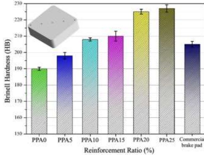
Figure 3. Effect of PPA content on the Brinell hardness of the developed brake pad composites
