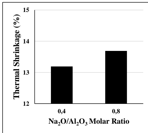
Figure 2. Thermal shrinkage values of the samples after heat treatment at 1050°C.
