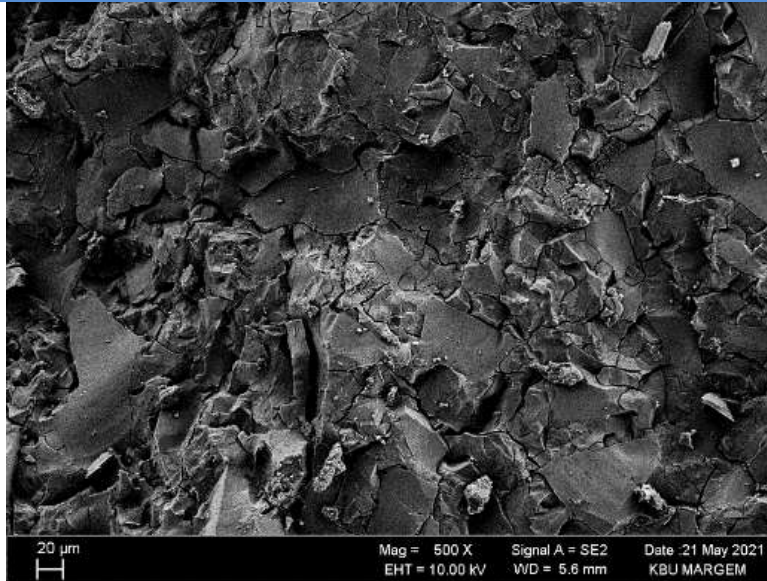
Figure 5. SEM image of the sample produced with with 4% silica addition.
