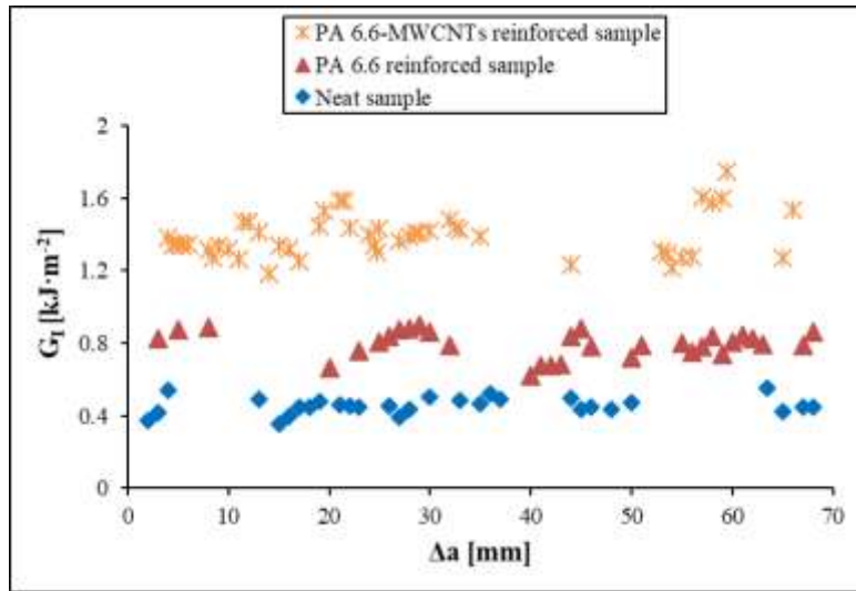
Figure 5. Mode-I interlaminar fracture toughness values of neat and reinforced carbon fabric/epoxy composite specimens.
