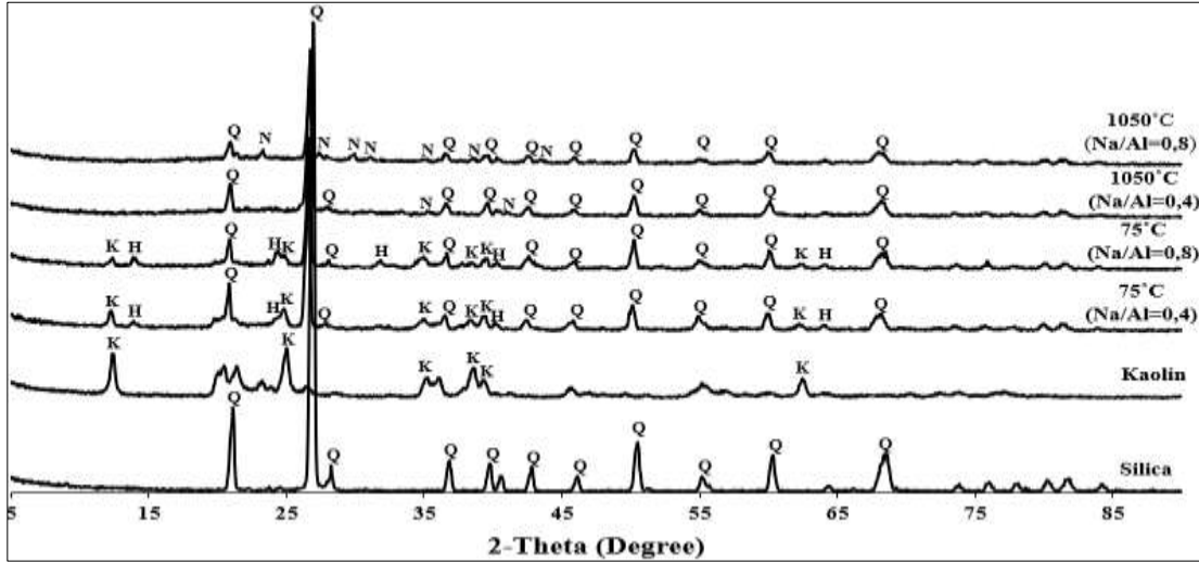
Figure 3. XRD patterns of the samples at different temperatures and with varying \text{Na}_2\text{O}/\text{Al}_2\text{O}_3 molar ratios.
