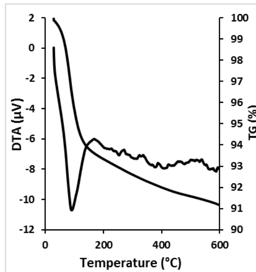
Figure 4. DTA-TG curve of the sample with 4% silica addition.
