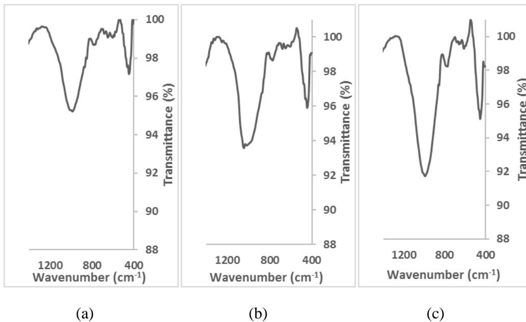
Figure 3. FT-IR spectra of samples with different % wt.silica addition levels; a)2, b)4, c)6.
