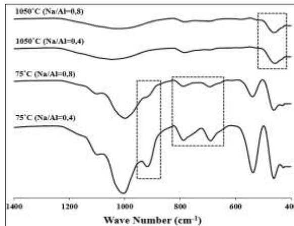
Figure 4. FTIR patterns of the samples produced at different temperatures and with varying \text{Na}_2\text{O}/\text{Al}_2\text{O}_3 molar ratios.
