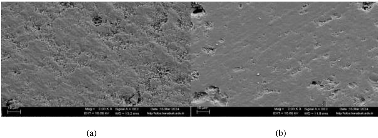
Figure 6. SEM images of samples heat-treated at 1050°C with varying Na 2 O/Al 2 O 3 molar ratios; a) 0.4, b) 0.8.
