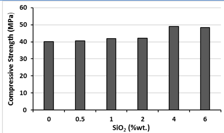
Figure 1. Compressive strengths of samples produced with different silica addition.
