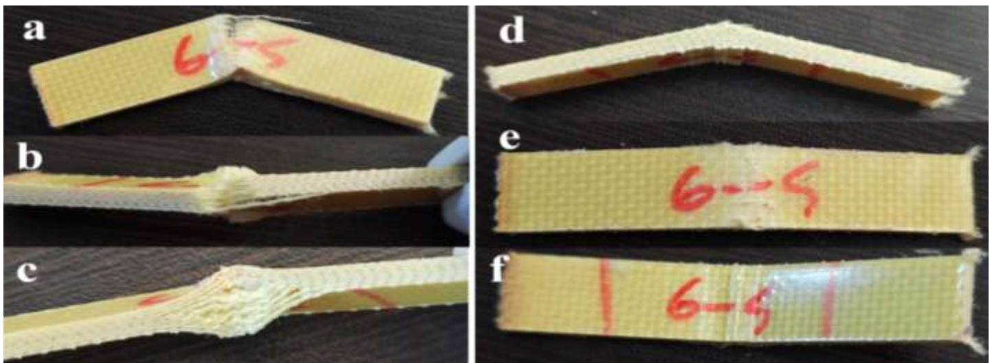
Figure 3. Images of samples after impact test; a, b, and c: horizontal samples, d, e and f: vertical samples
