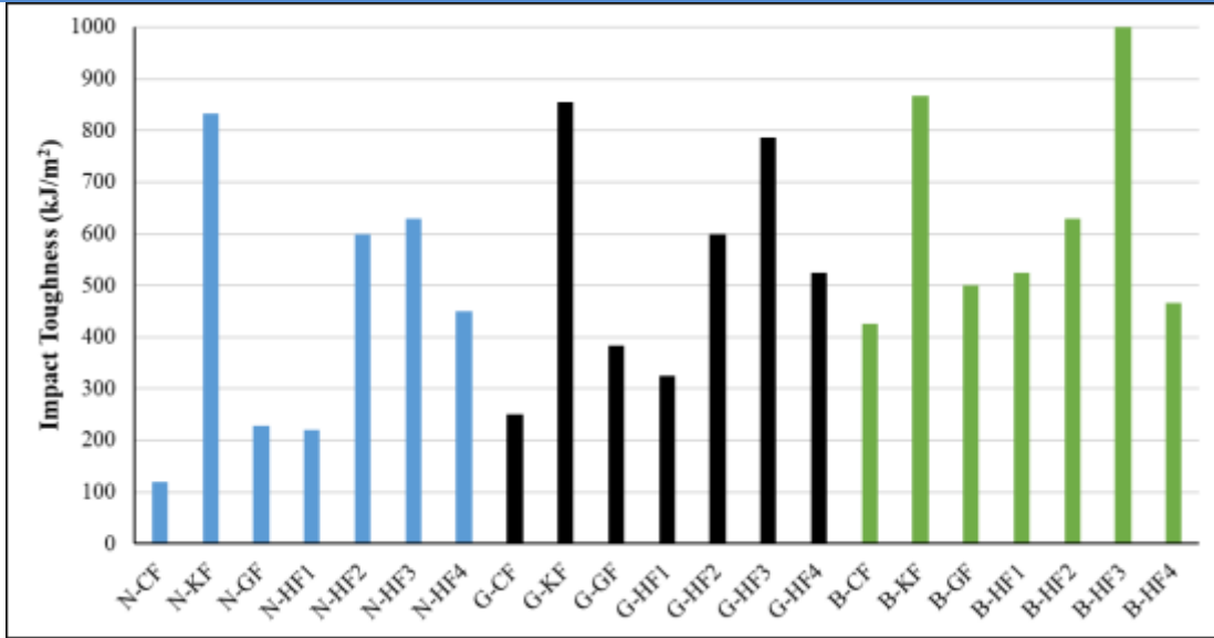
Figure 2. Fracture toughness values obtained from the Charpy impact tests
