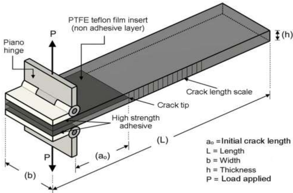
Figure 2. Mode-I interlaminar fracture toughness test specimen (Sharma, 2021).
