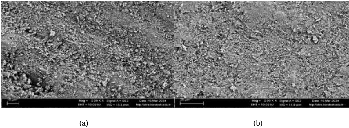
Figure 5. SEM images of samples heat-treated at 75°C with varying Na 2 O/Al 2 O 3 molar ratios; a) 0.4, b) 0.8.
