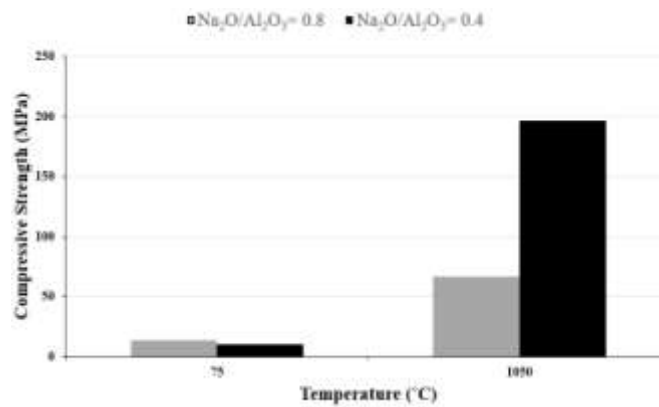
Figure 1. Compressive strength of samples with varying \text{Na}_2\text{O}/\text{Al}_2\text{O}_3 molar ratios at different temperatures.
