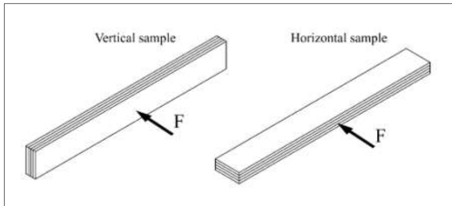
Figure 1. Horizontal and vertical samples and application of impact
